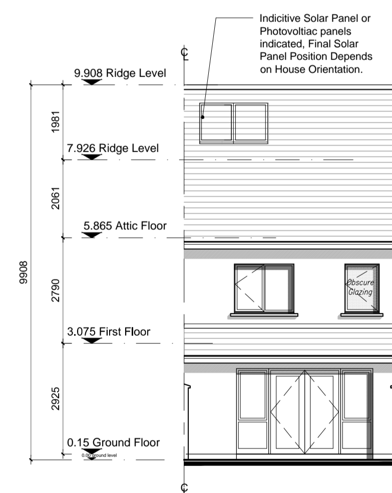
Rear Elevation 'C' Left Entry
