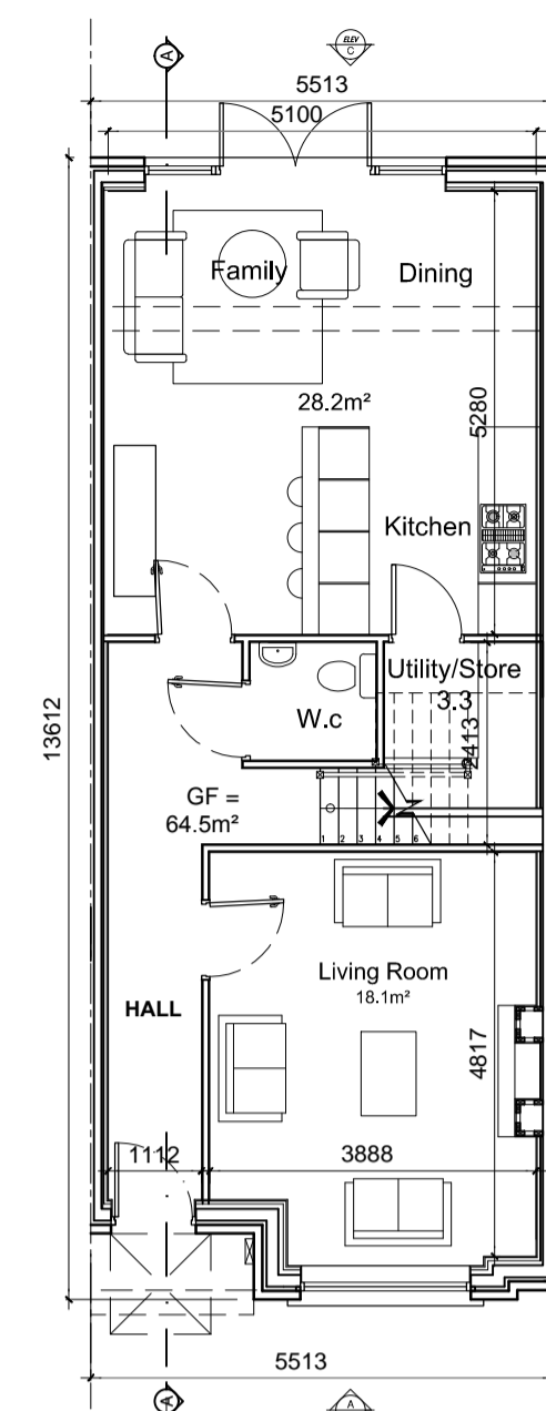
Ground Floor Plan Left Entry area 64.5m 2 / 694 ft 2 O/ALL AREA 119m 2 / 1280ft 2
