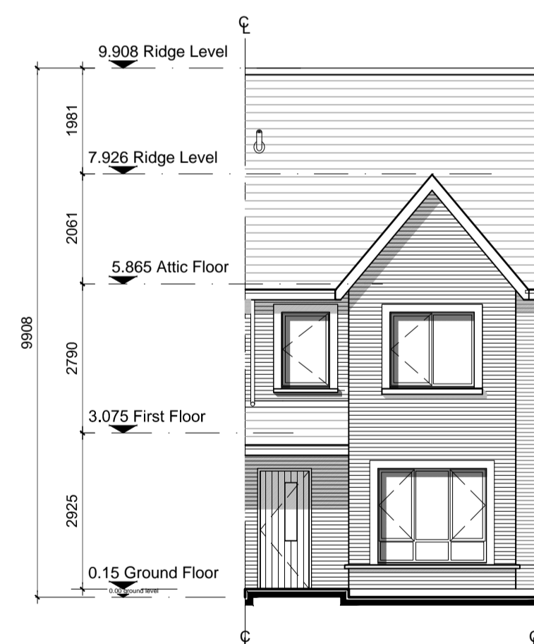
Front Elevation 'A' Left Hand Entry
