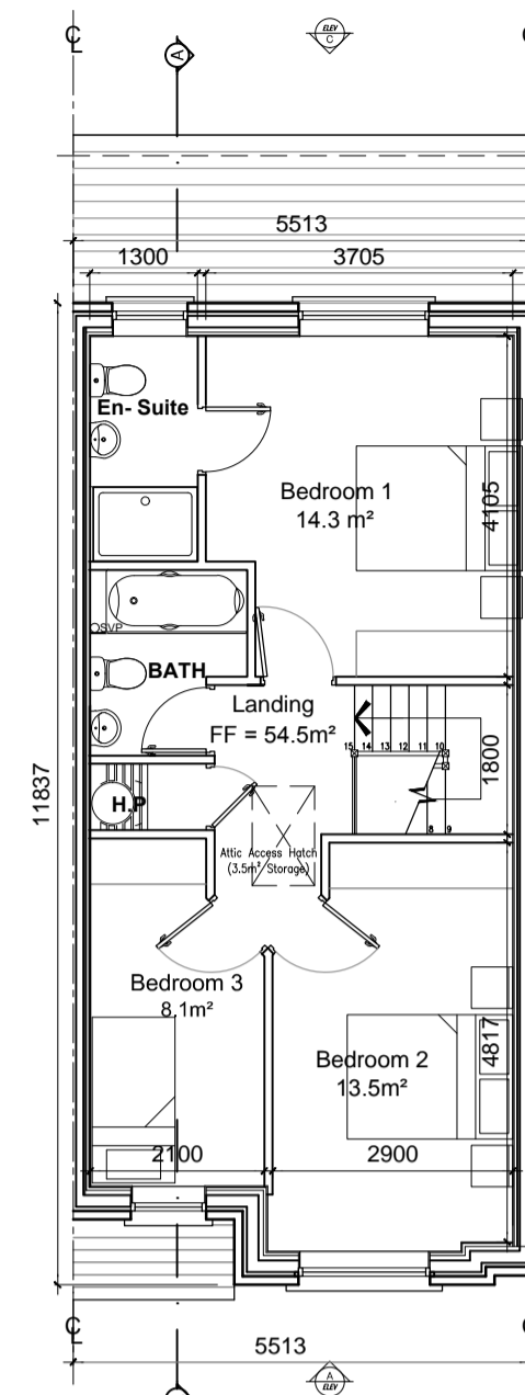
First Floor Plan Left Entry area 54.5m 2 / 586 ft 2
